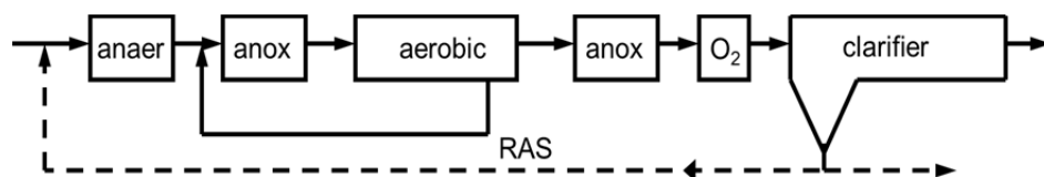
Fig. 7. Bardenpho-Process
