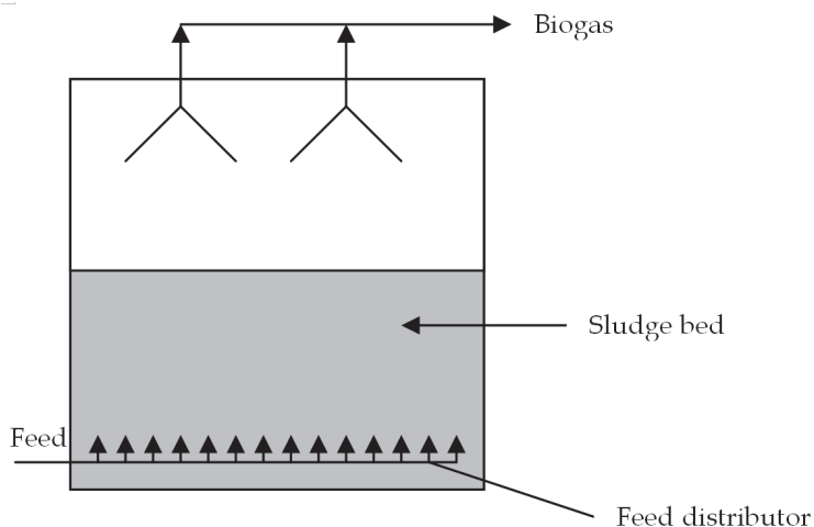
Fig. 5. Upflow anaerobic sludge blanket reactor (adapted from Khanal, 2008)
