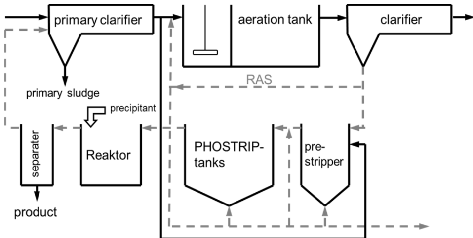
Fig. 16. PHOSTRIP-Process
