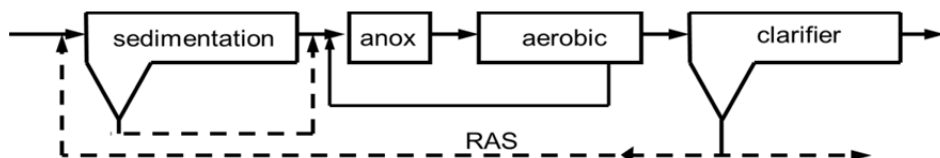
Fig. 13. Extended Anaerobic Sludge Contact (EASC) Process
