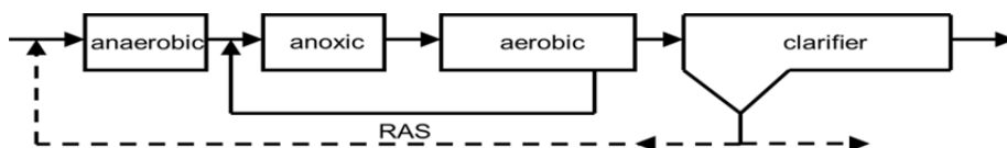
Fig. 9. Phoredox-Process
