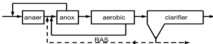
Fig. 8. UCT-Process
